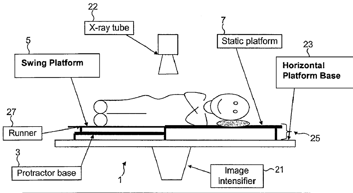
Passive Motion Platform - Side Elevation
