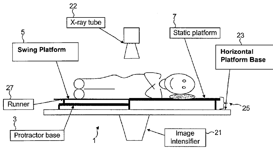
Passive Motion Platform - Side Elevation
