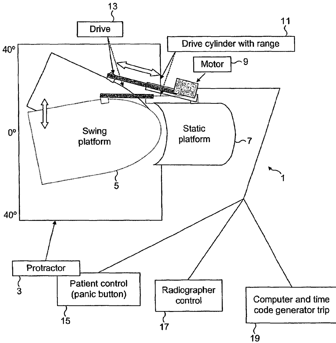
Passive Motion Platform - Top Elevation
